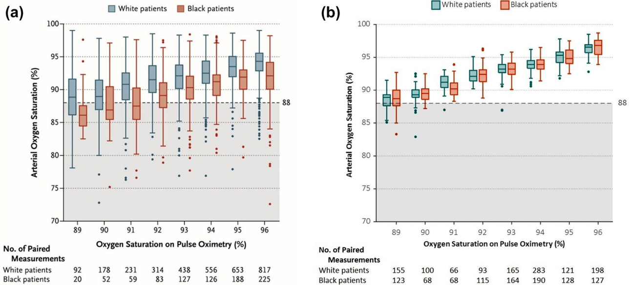
Fig. 3 Box plots showing accuracy comparison for Black (salmon tint) and White (blue tint) ethnic groups binned by 1% saturation bins, from 89–96%. Figure 3a reproduced (with permission) from the Sjo-
