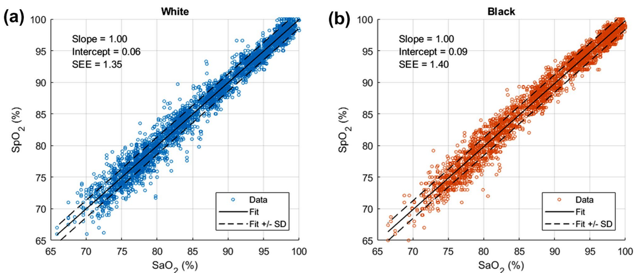
Fig. 2 Scatter plot ( \text{SpO}_2 versus \text{SaO}_2 ) along with performance metrics for White subjects (Fig. 2a) vs. Black subjects (Fig. 2b)
